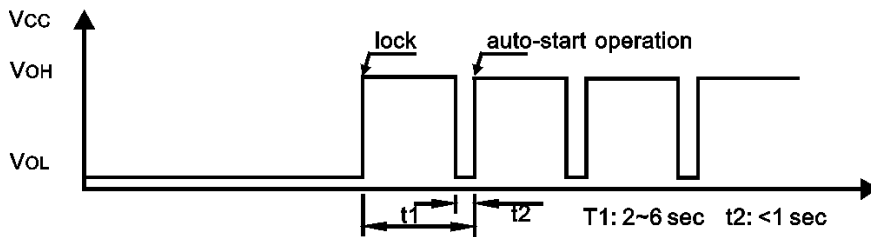
Output Waveform
