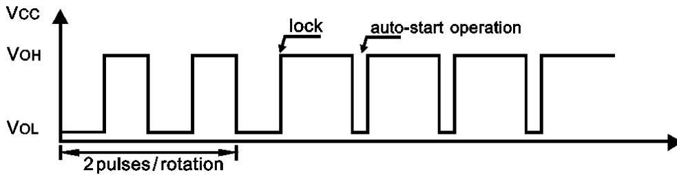
Output Waveform
