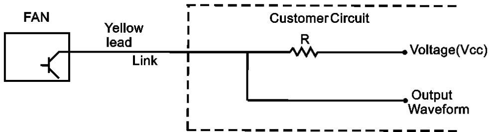
Output Waveform
