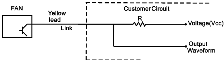
Output Waveform
